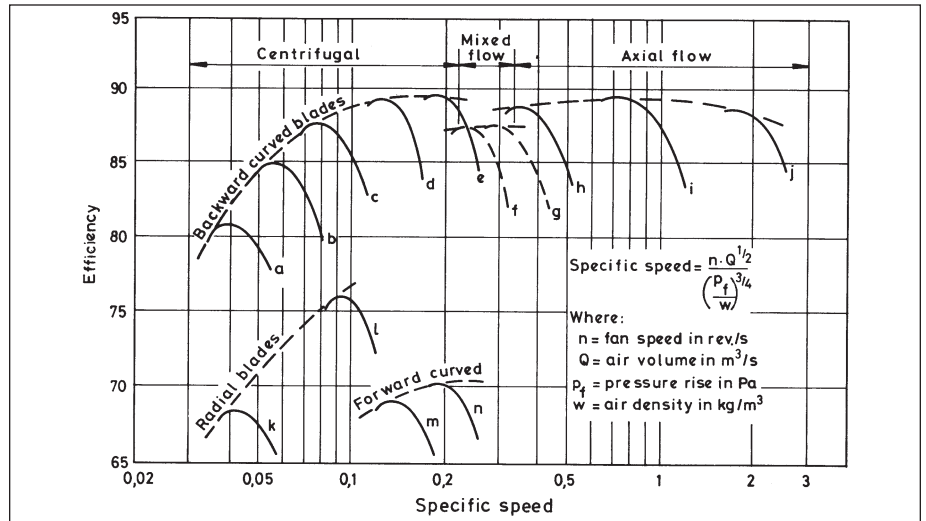
Fig. 2. Fan efficiency vs specific speed (environmental engineering in South African mines, 1989).
