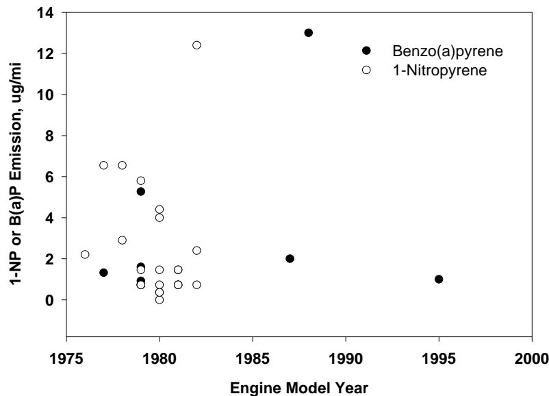
Figure 2-37. Diesel engine emissions of benzo[ a ]pyrene and 1-nitropyrene measured in chassis dynamometer studies.
