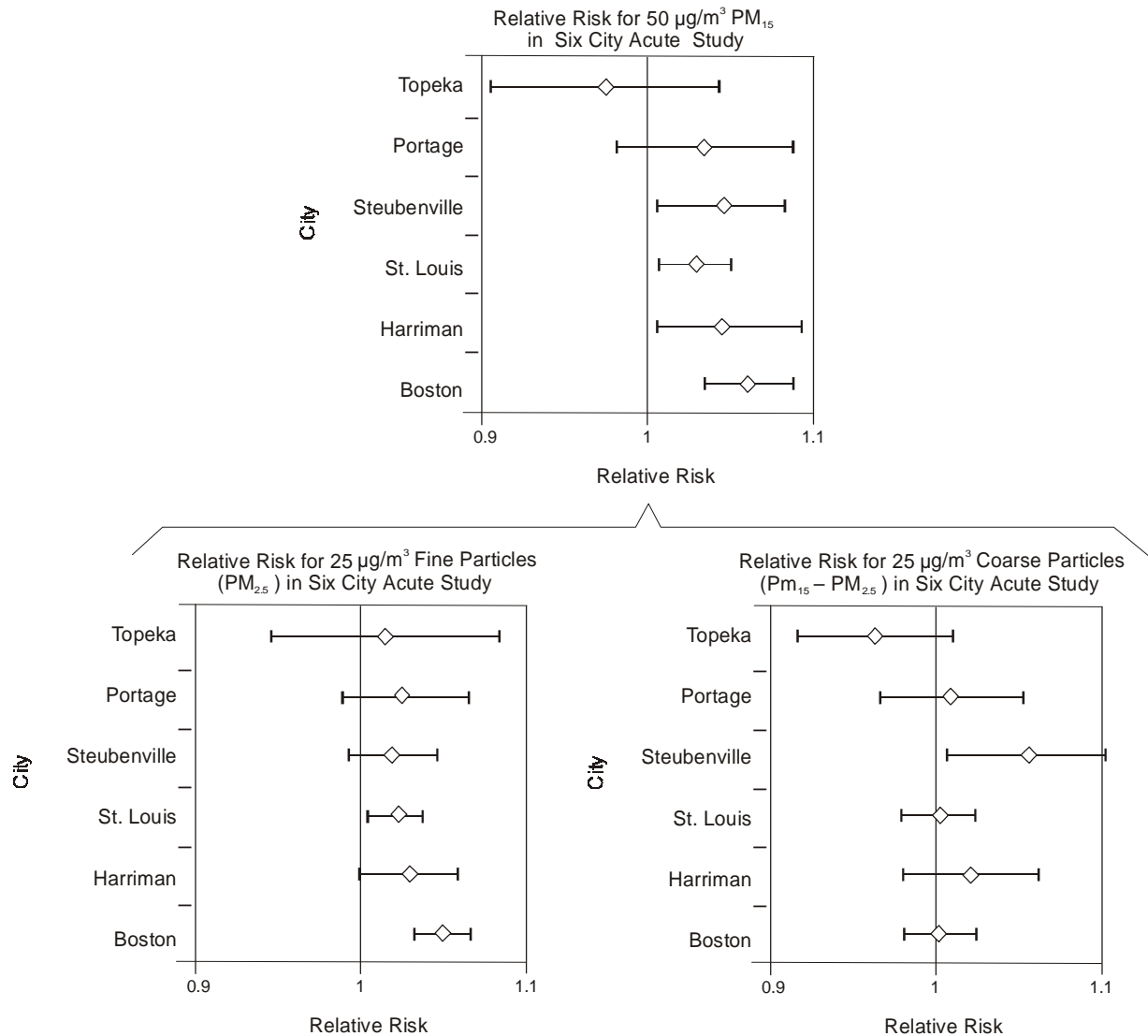
Figure 6-3. Relative risks of acute mortality in Harvard Six Cities Study, for inhalable thoracic particles (PM 15 /PM 10 ), fine particles (PM 2.5 ), and coarse fraction particles (PM 15 -PM 2.5 ).
