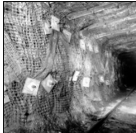
Rib side with GRP bolts
