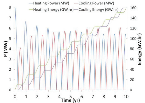
Fig. 4. Heating/cooling power and their associated energy savings
